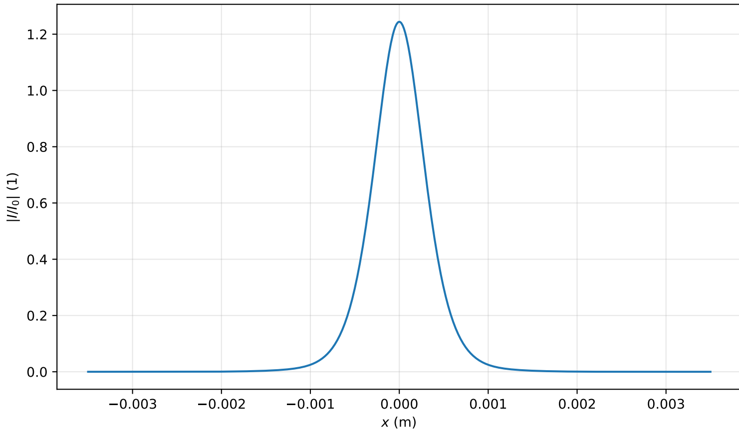
Intensity profile I(x, y = 0, z = 2.388m)/I_0 , P_{in}=0.8P_{cr} , artificial time
